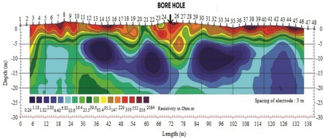
Fig. 2 Soil layer profile of survey line
