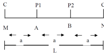
Fig. 1 Current and potential electrodes in the Wenner configuration
